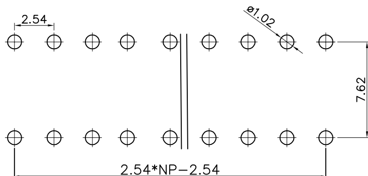
PCB LAYOUT
