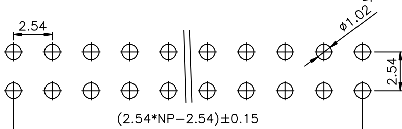
PCB LAYOUT
